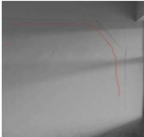
Photograph4: Joint of column-wall and Beam-wall (Diagonal cracks)
