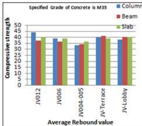
Figure 4: Graph of Rebound number v/s Compressive strength
