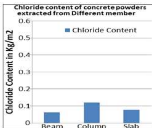
Figure 6: Chloride content of concrete (Taken average value of beam, column and slab)
